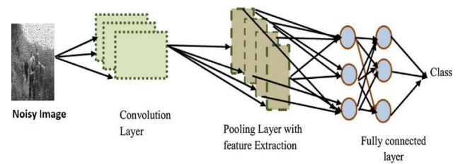
Fig3:Convolutionneuralnetworkmodel
