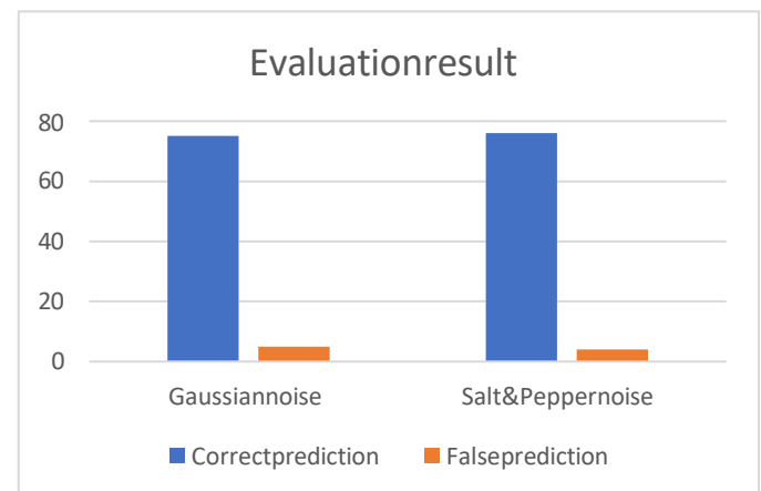
Fig5:Graphofevaluation results
