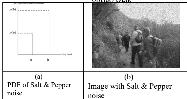
Fig2:Salt&pepperNoisemodel
